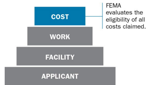
Figure 8. Cost Eligibility
